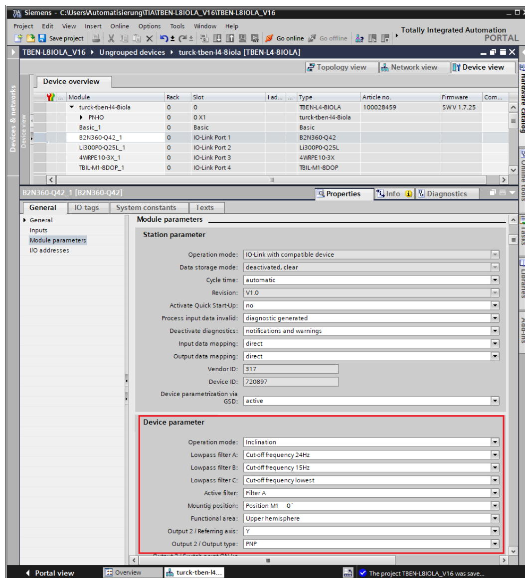
Fig. 86: Example: TIA Portal, IO-Link device parameters via GSDML
