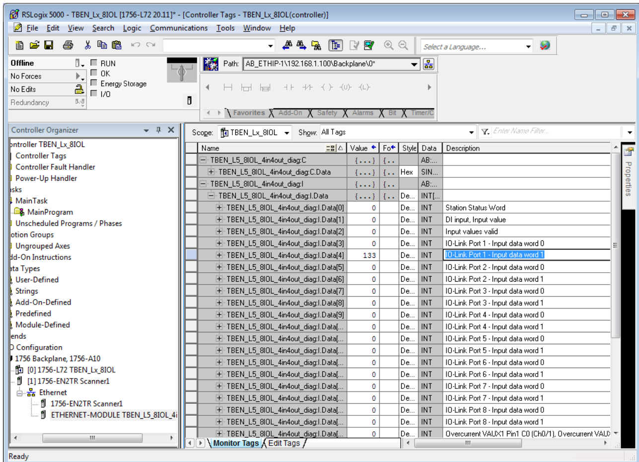
Fig. 66: Controller Tags in the project tree
