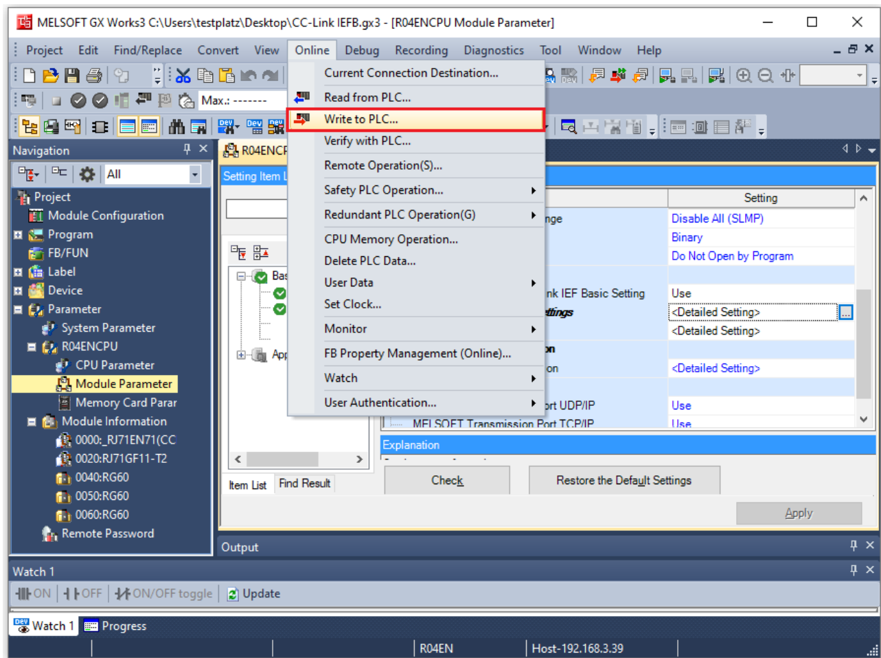
Fig. 77: GX Works3: Writing the configuration to the PLC
