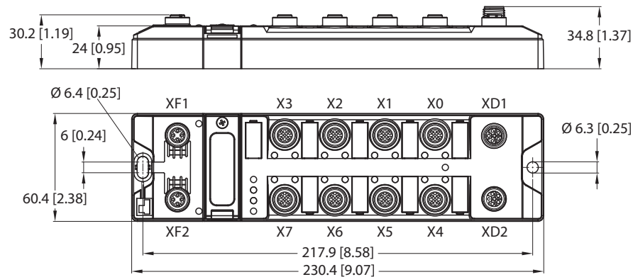
Fig. 1: Dimensions TBEN-LL-8IOL
