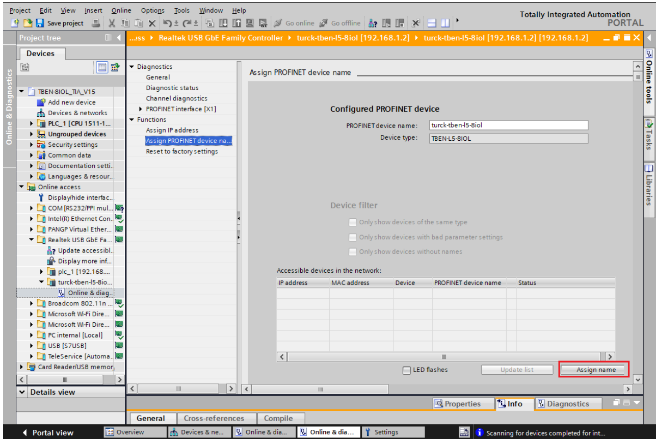
Fig. 34: TIA-Portal: Assigning the PROFINET device name
