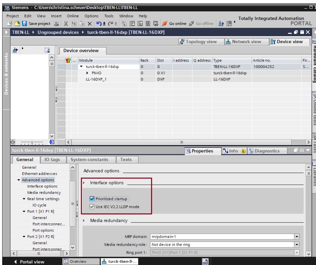
Fig. 30: TIA-Portal – prioritized start-up, activation at the I/O device
