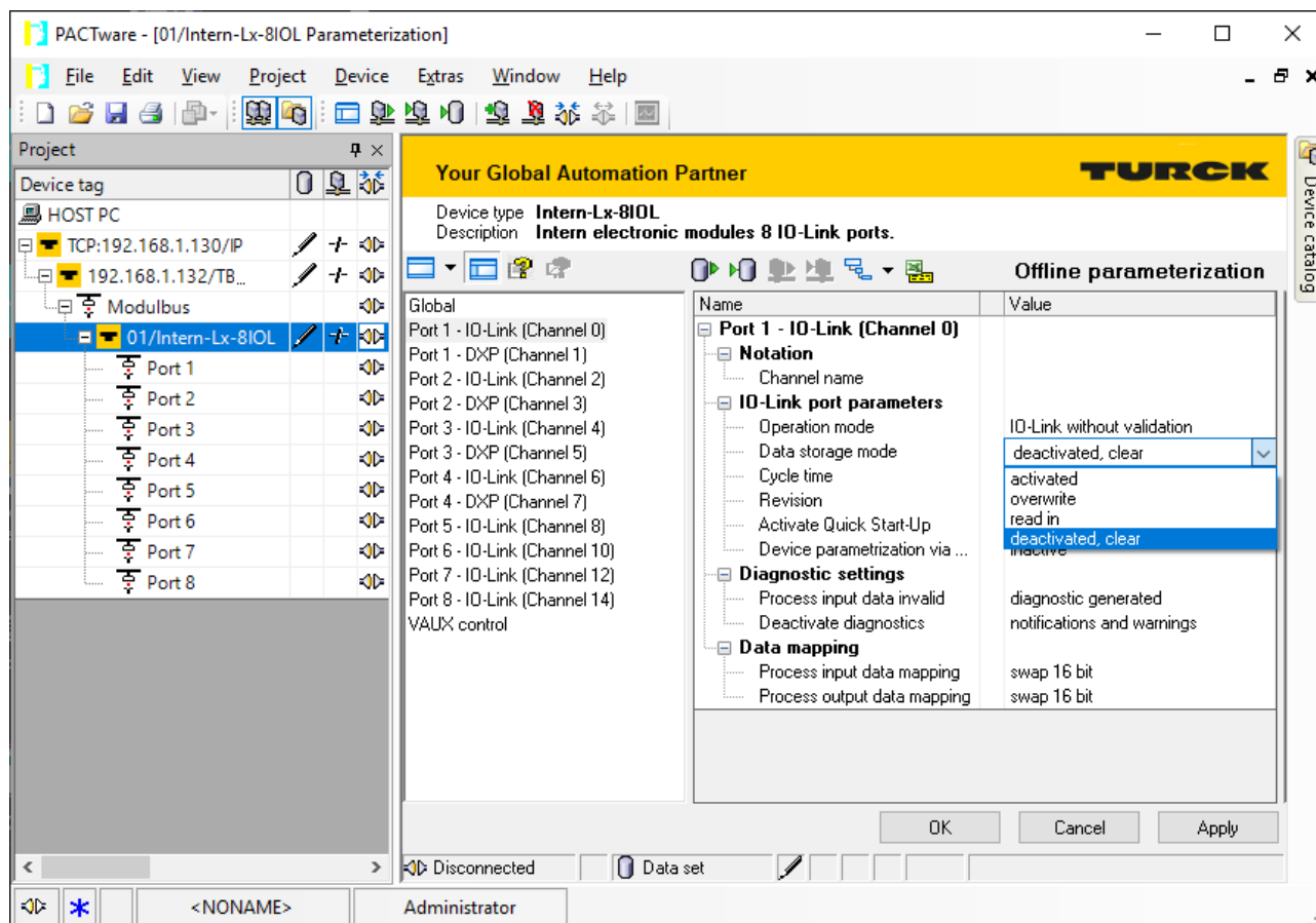
Fig. 90: Example: Deactivate or respectively delete the data storage mode with the DTM
