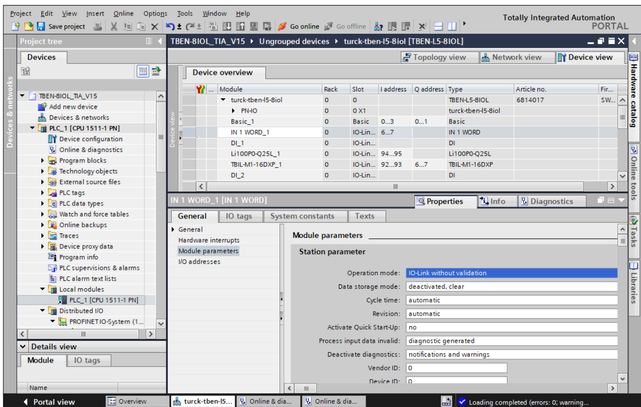
Fig. 37: TIA-Portal: parameterizing generic IO-Link devices
