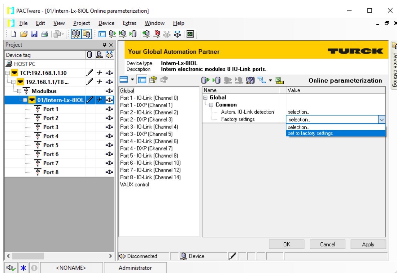
Fig. 91: Example: Reset device to factory settings via DTM
