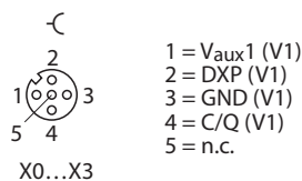
Fig. 20: Pin assignment of IO-Link master ports, Class A, X0...X3
