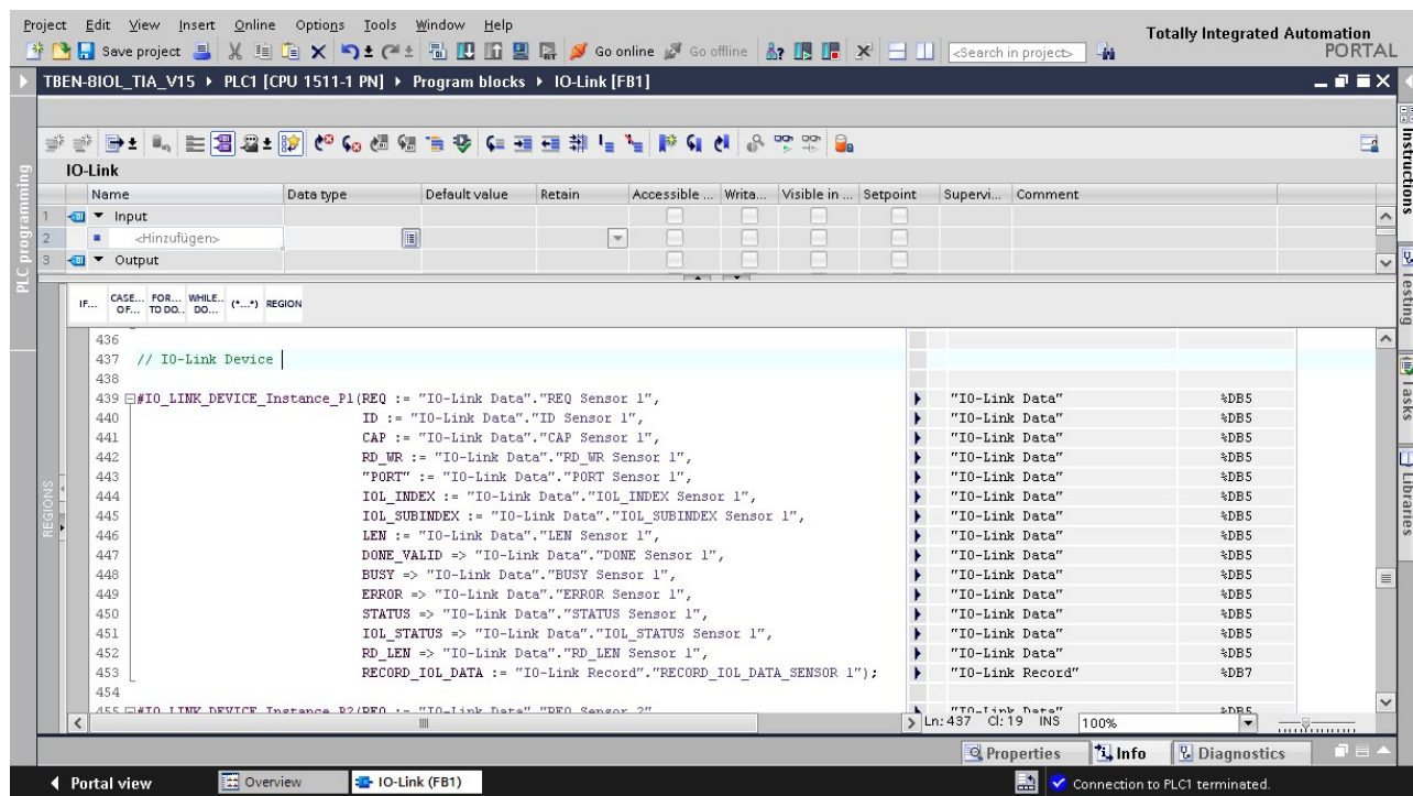
Fig. 39: Example call of Siemens FB "IO_LINK_DEVICE"
