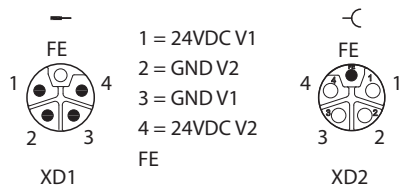
Fig. 17: Pin assignment power supply connectors
