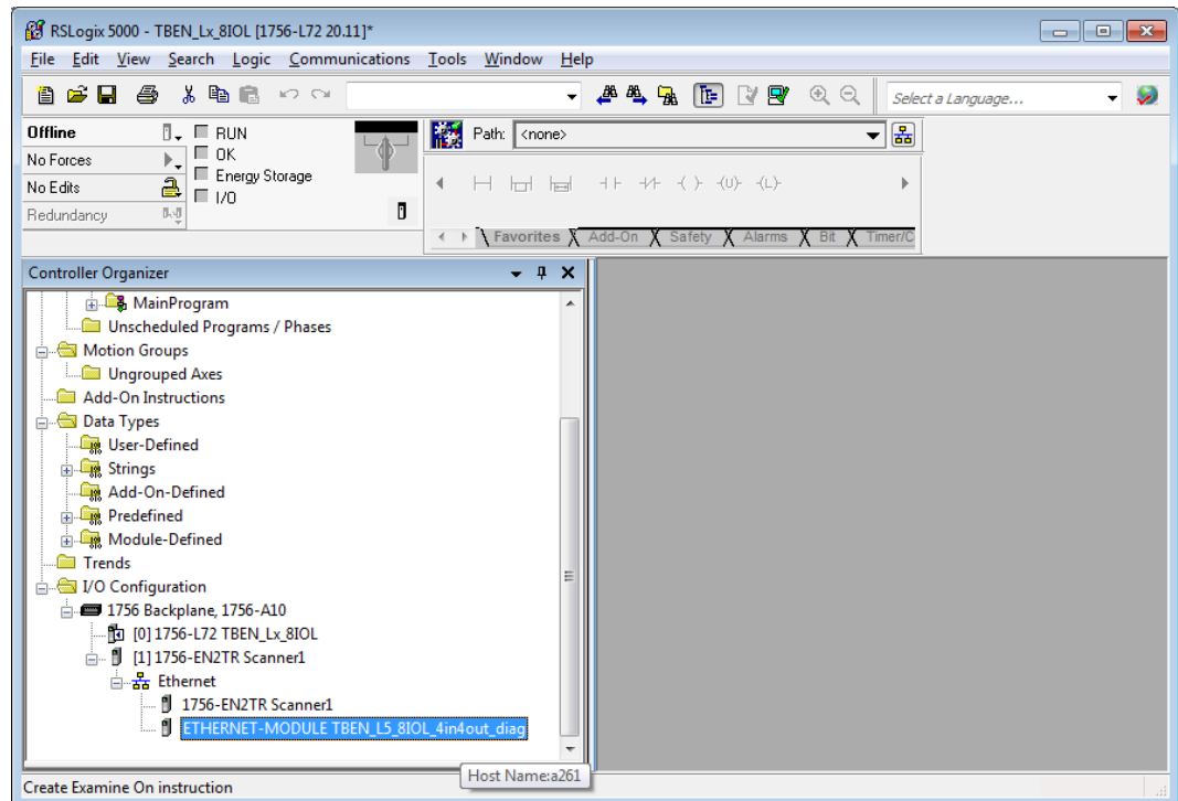
Fig. 60: Predefined configurations of TBEN-L...-8IOL in new project
