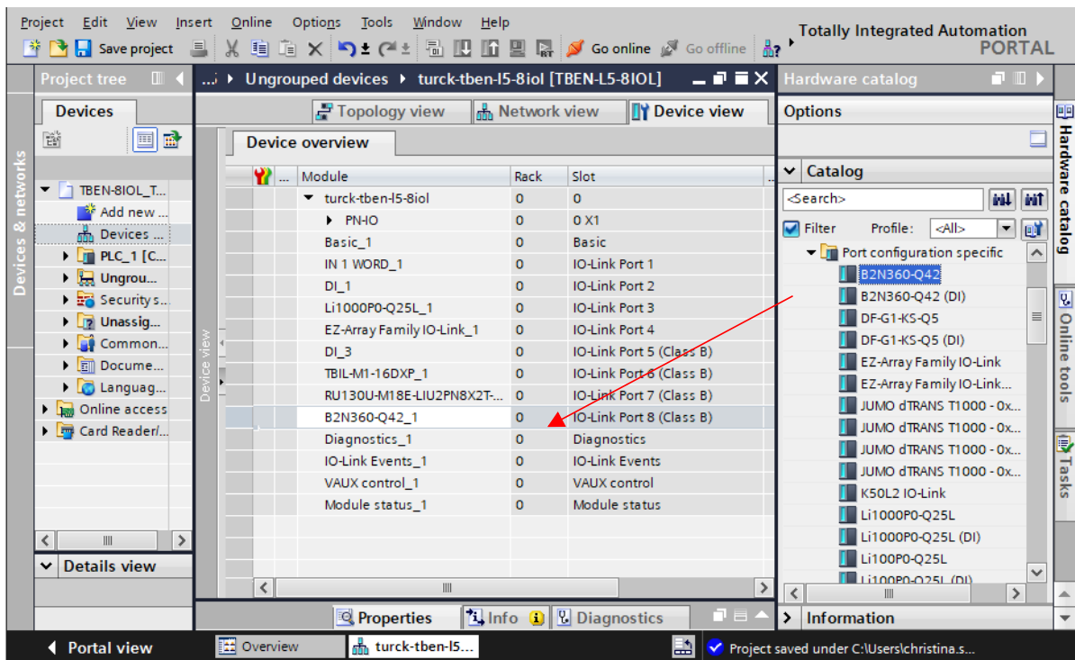
Fig. 36: TIA-Portal: Configuring device slots
