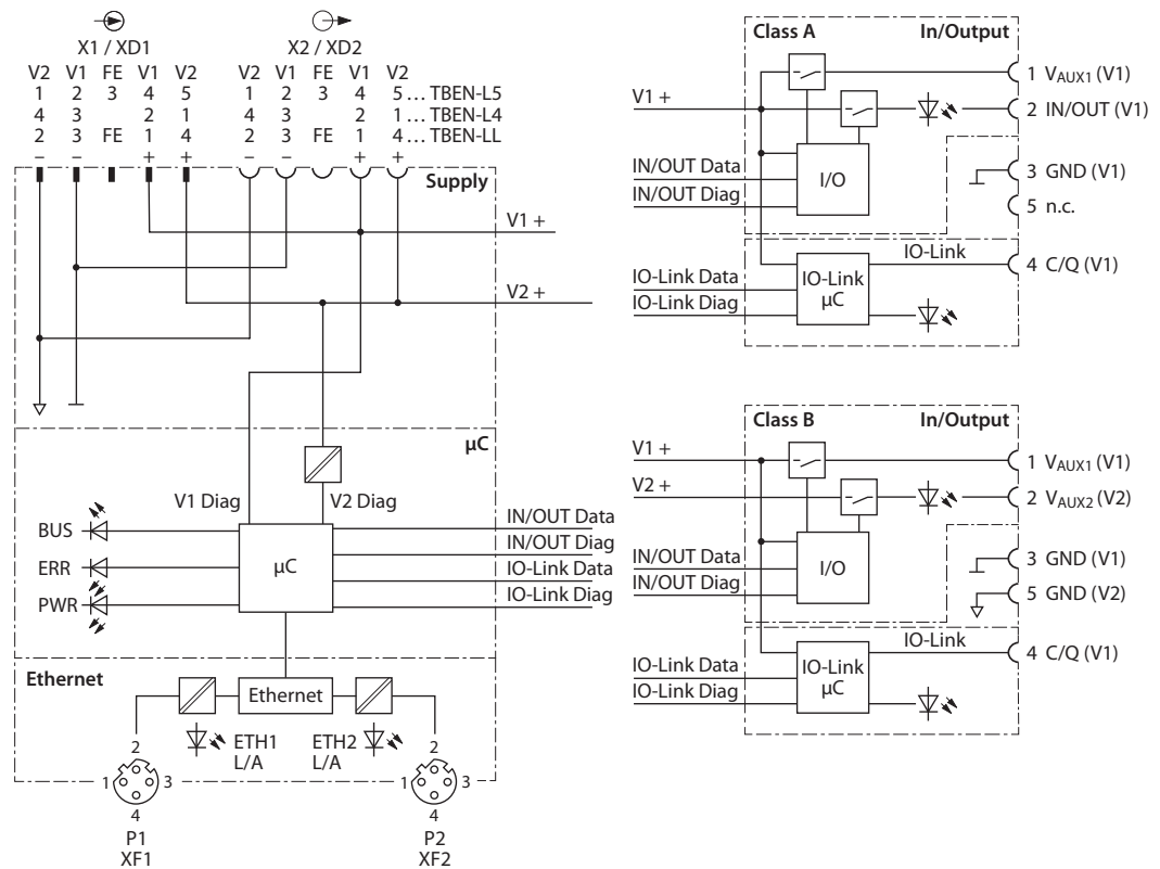
Fig. 2: Block diagram
