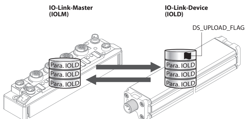
Fig. 94: Data storage mode – general principle, Para. IOLD = parameters of the IO-Link device
