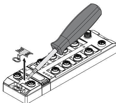
Fig. 12: Removing the grounding clamp
