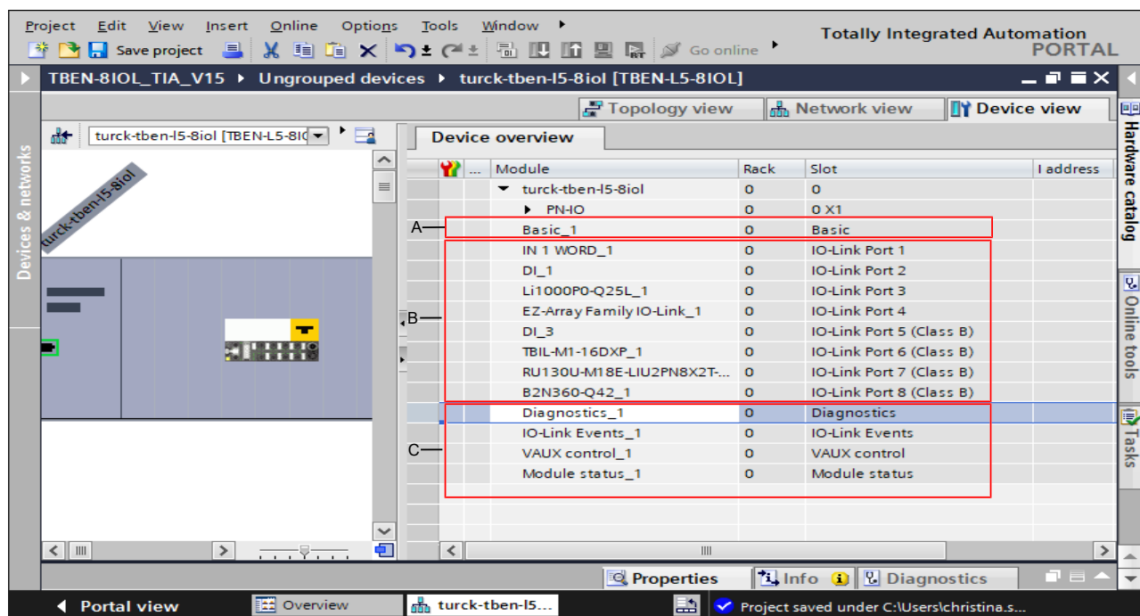
Fig. 28: TBEN-L...-8IOL: slot overview in TIA-Portal (example)
