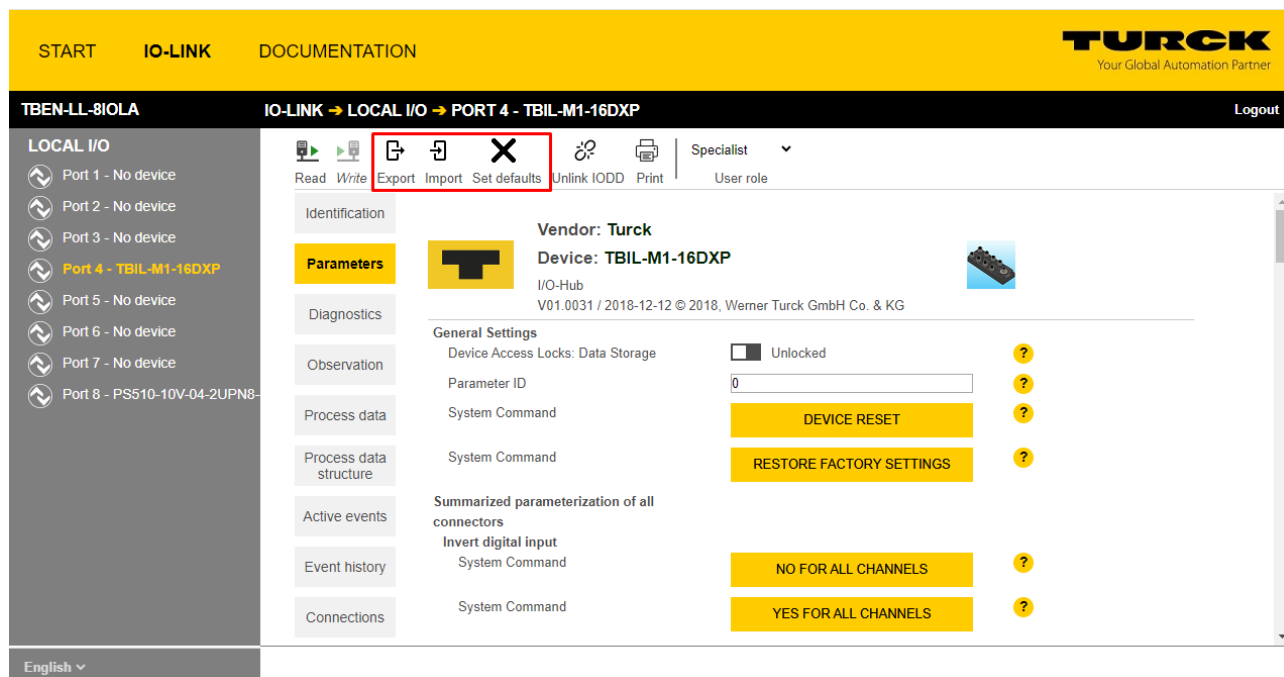
Fig. 83: Parameters of the IO-Link device
