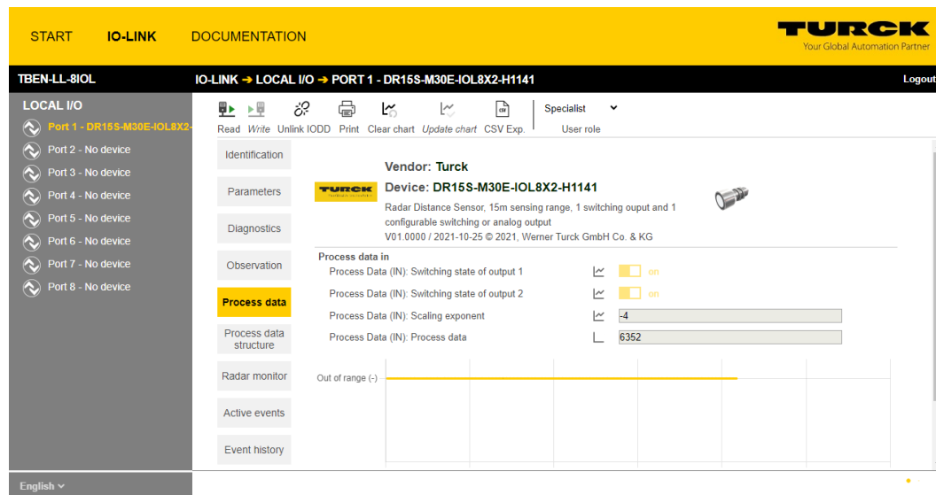
Fig. 101: Process data of an IO-Link device
