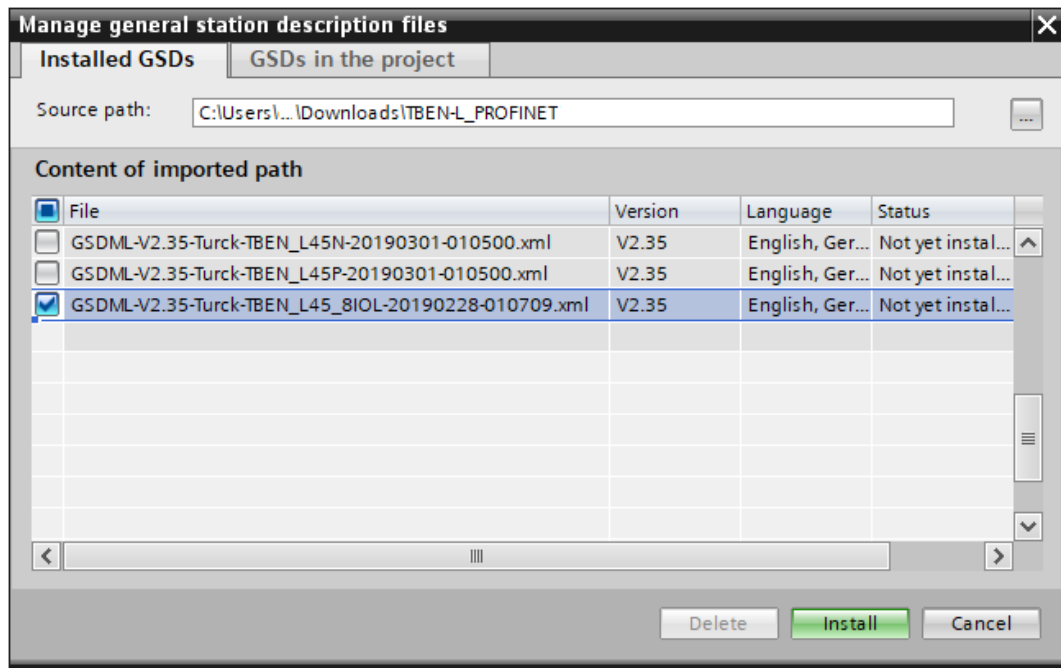
Fig. 32: TIA Portal: Installing the GSDML-file
