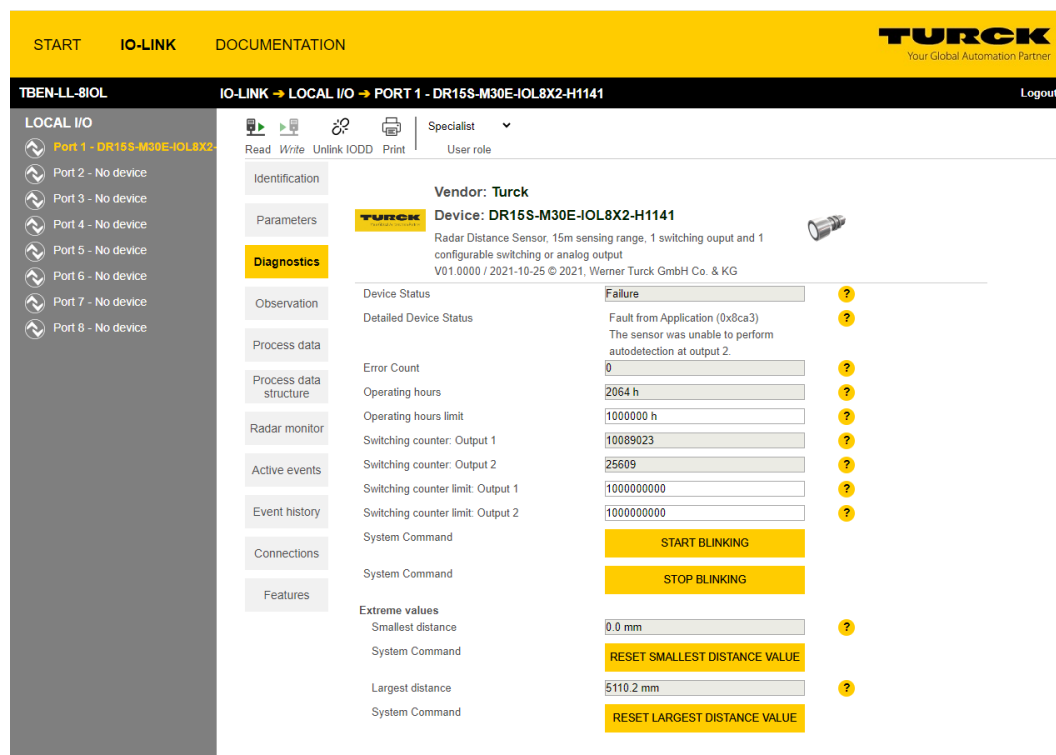
Fig. 102: Diagnostics at IO-Link device
