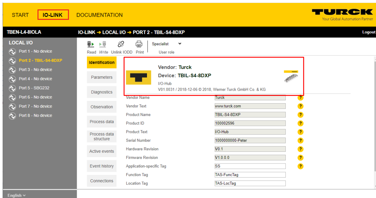
Fig. 82: IO-Link device with device specific IODD
