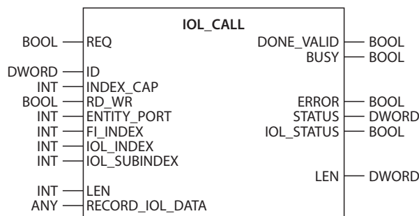
Fig. 31: IOL_CALL in accordance with IO-Link specification
