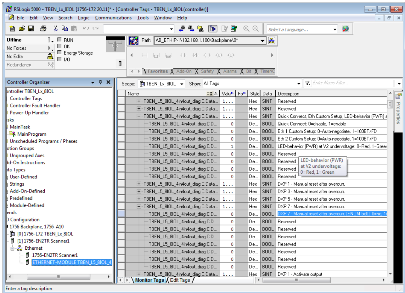
Fig. 63: Parameterizing the device
