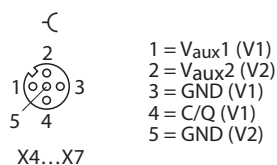
Fig. 21: Pin assignment of IO-Link master ports, Class B, X4...X7
