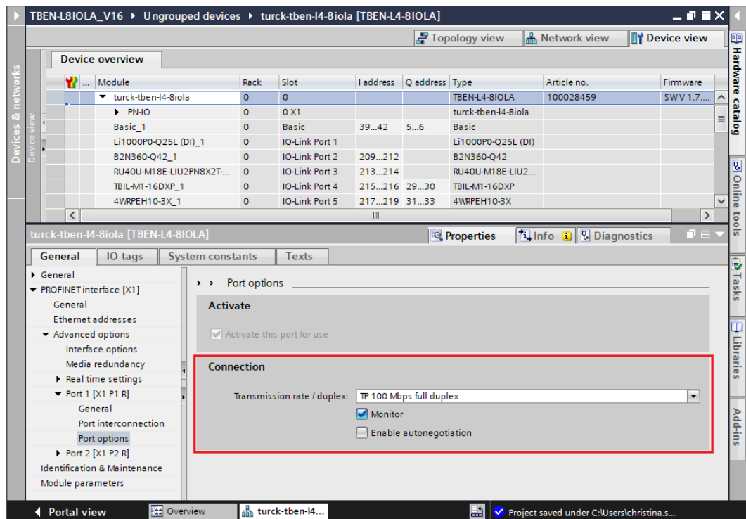
Fig. 29: TIA-Portal – port-settings for FSU
