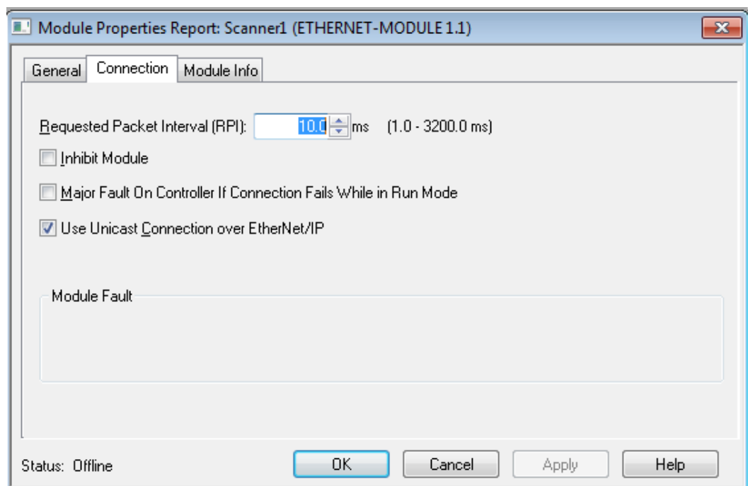
Fig. 62: Setting the connection parameters
