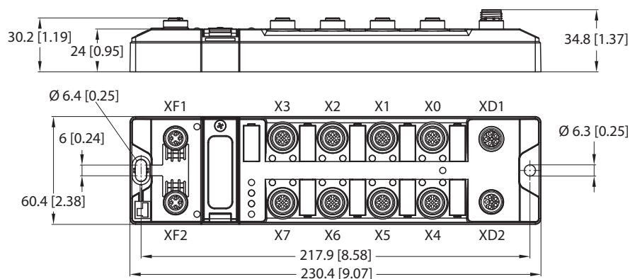
Fig. 2: Dimensions TBEN-LL-8IOLA
