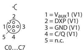
Fig. 27: Pin assignment of IO-Link master ports C0...C7, Class A
