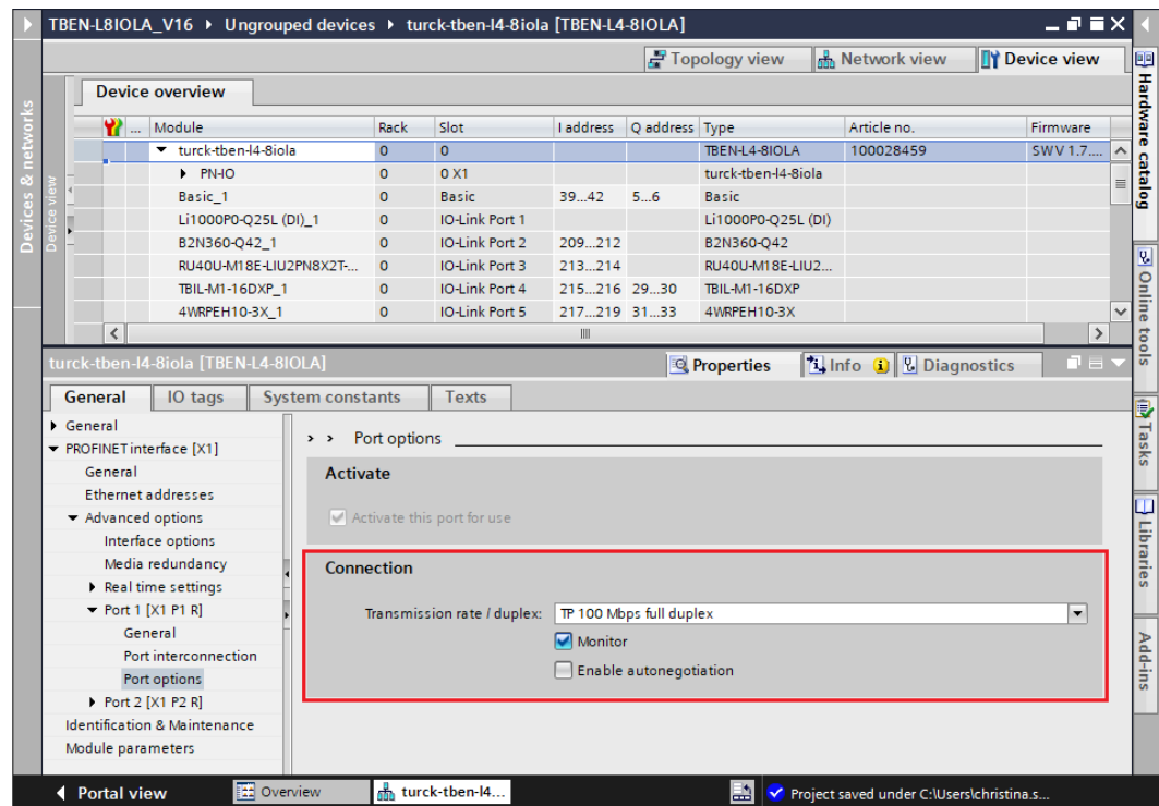
Fig. 36: TIA-Portal – port-settings for FSU
