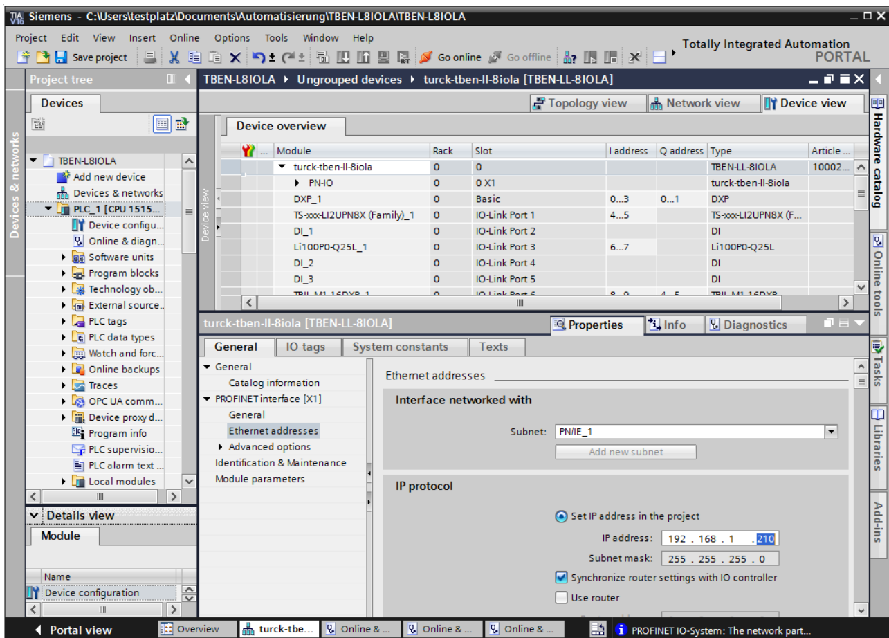
Fig. 42: TIA-Portal: Assigning the IP address
