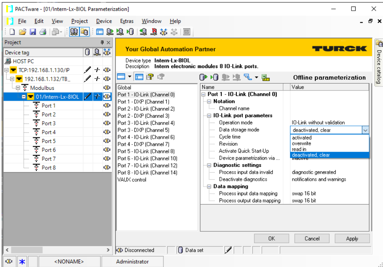
Fig. 102: Example: Deactivate or respectively delete the data storage mode with the DTM
