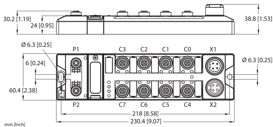
Fig. 1: Dimensions TBEN-L4-8IOLA
