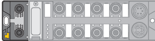
Fig. 16: M12 Ethernet connector
