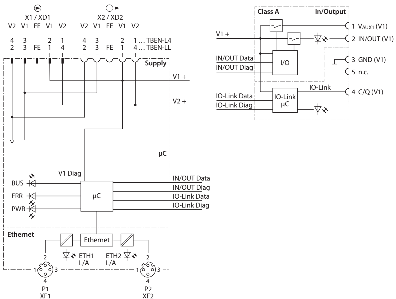
Fig. 3: Block diagram
