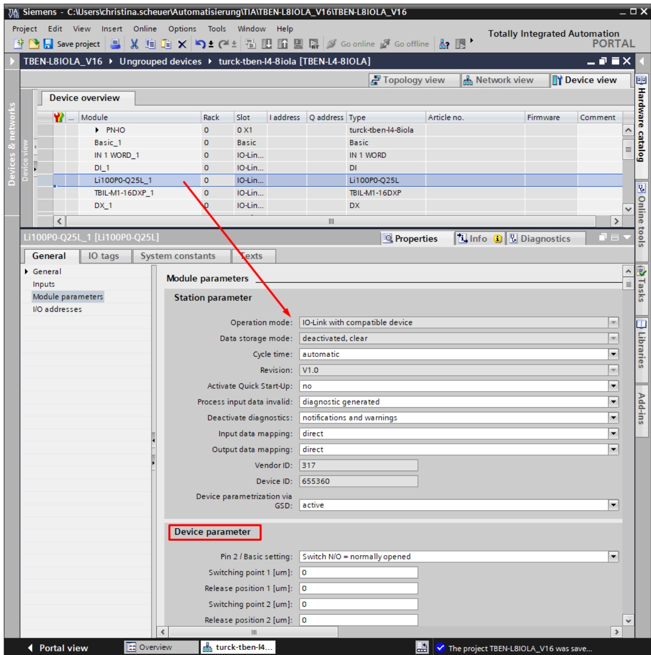
Fig. 45: TIA-Portal – IO-Link port with specific configuration (SIDI)
