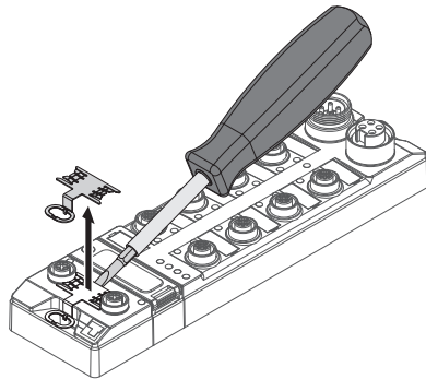
Fig. 13: Removing the grounding clamp
