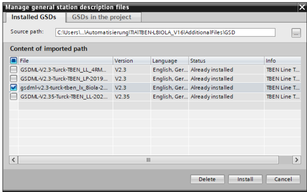
Fig. 39: TIA Portal: Installing the GSDML-file
