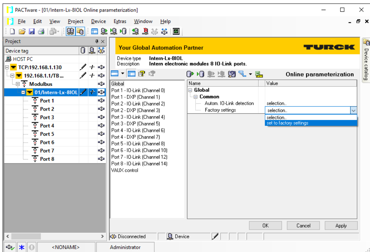
Fig. 101: Example: Reset device to factory settings via DTM
