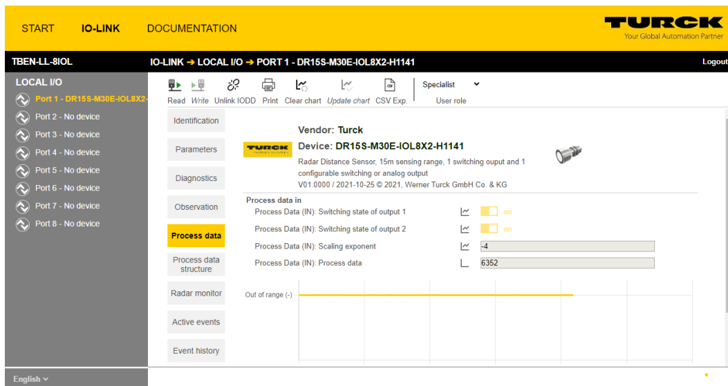
Fig. 111: Process data of an IO-Link device
