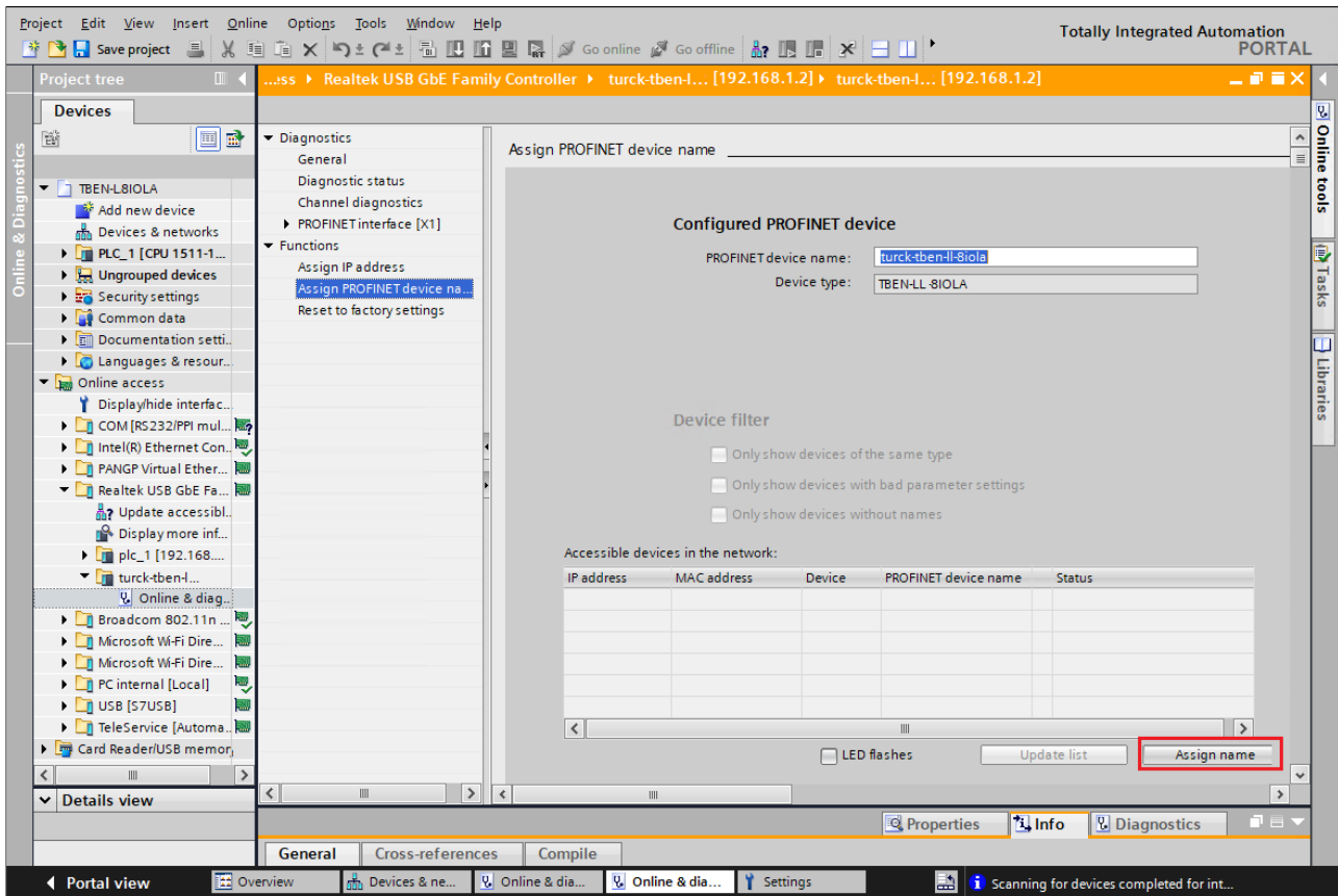
Fig. 41: TIA-Portal: Assigning the PROFINET device name
