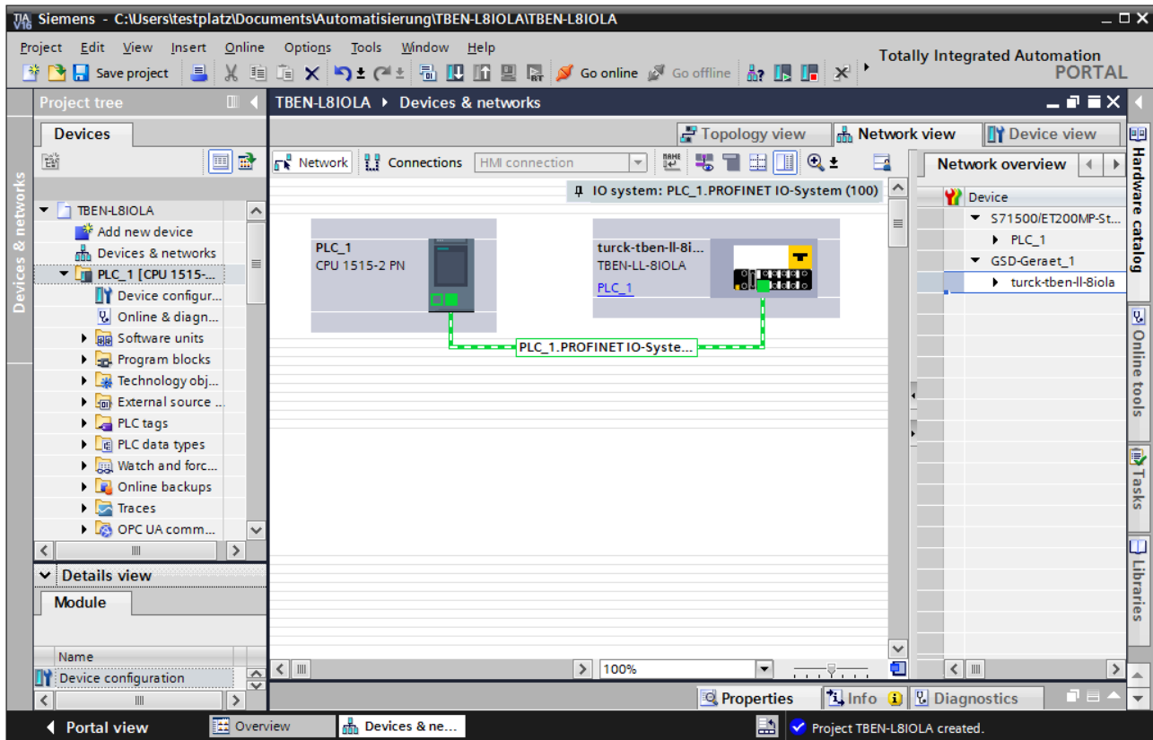
Fig. 40: Connecting the device to the PLC
