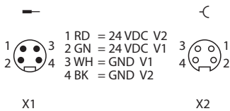
Fig. 21: TBEN-L4... – pin assignment power supply connectors
