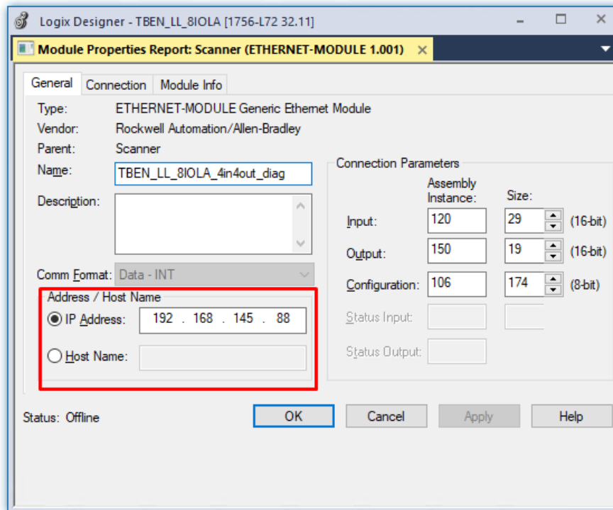
Fig. 71: Setting module name and IP address
