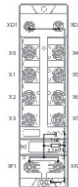
Fig. 11: TBEN-LL-8IOLA – equivalent wiring diagram and shielding concept
