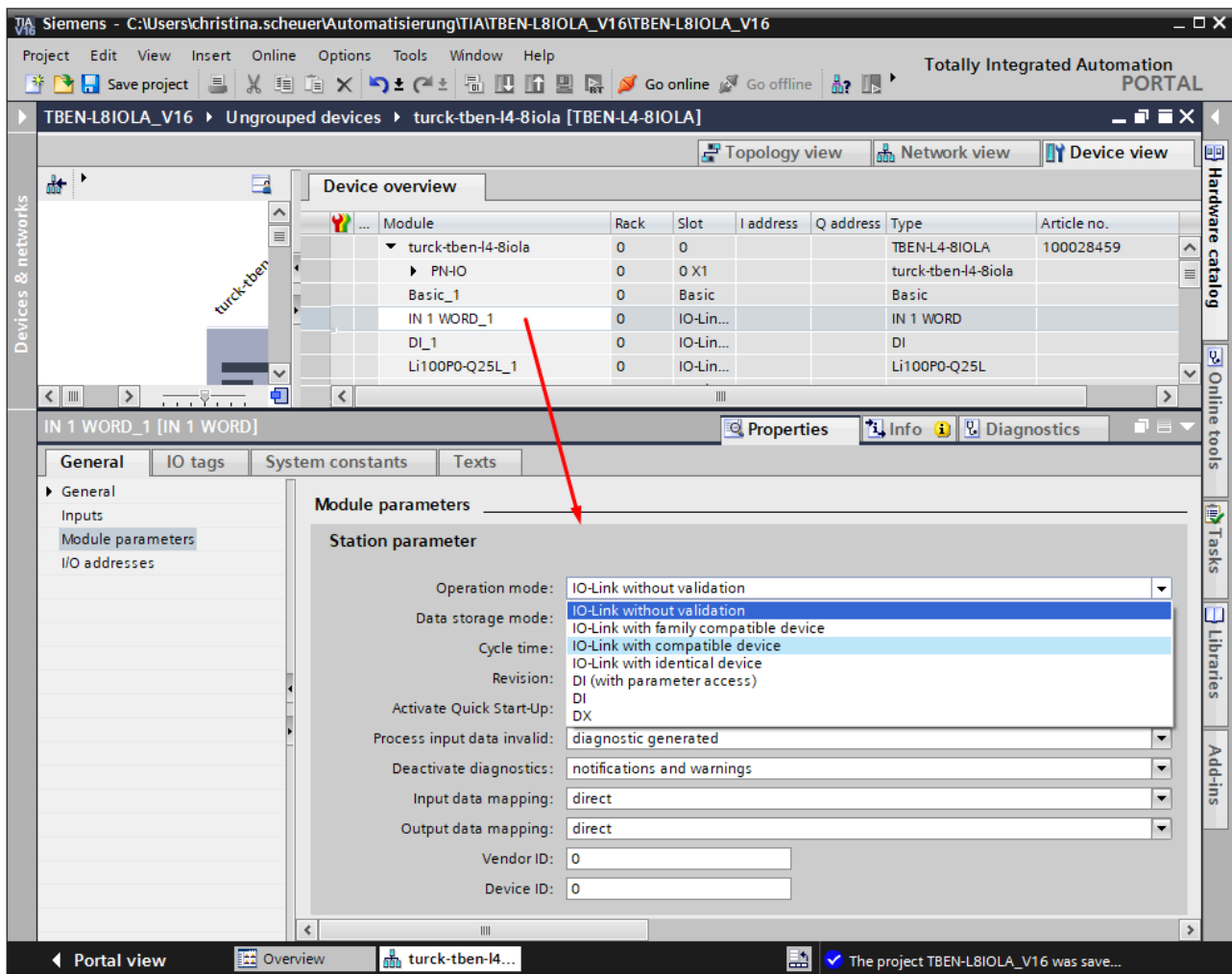
Fig. 44: TIA-Portal – IO-Link port with generic configuration
