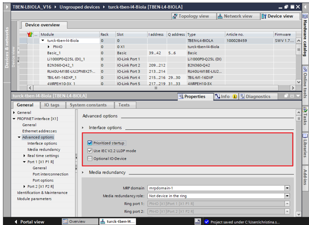
Fig. 37: TIA-Portal – prioritized start-up, activation at the I/O device
