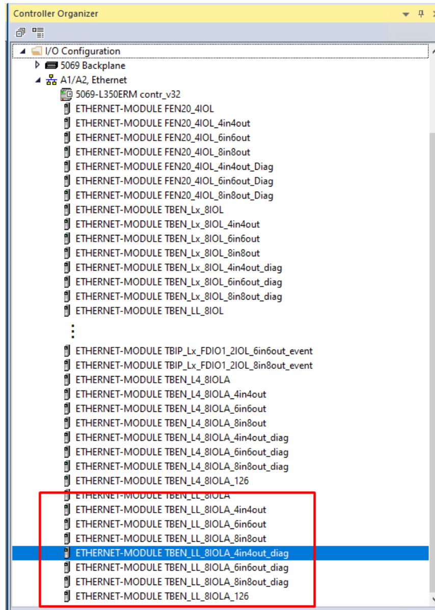
Fig. 69: Copying the device entry from catalog file
