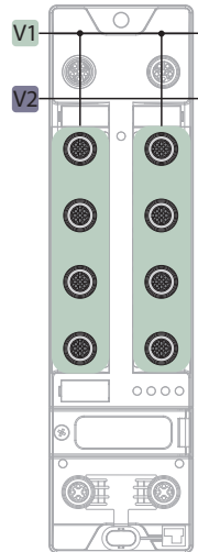
Fig. 24: Supply TBEN-LL-8IOLA
