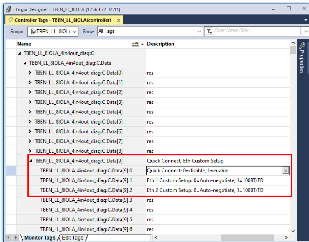
Fig. 67: Configuring QuickConnect in Logix Designer
