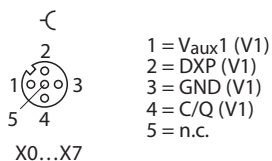
Fig. 28: Pin assignment of IO-Link master ports X0...X7, Class A
