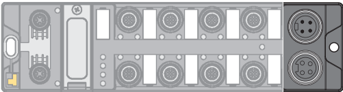
Fig. 20: TBEN-L4... – 7/8" connector for connecting the supply voltage
