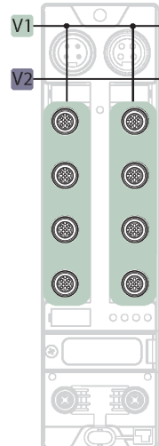
Fig. 25: Supply TBEN-L4-8IOLA
