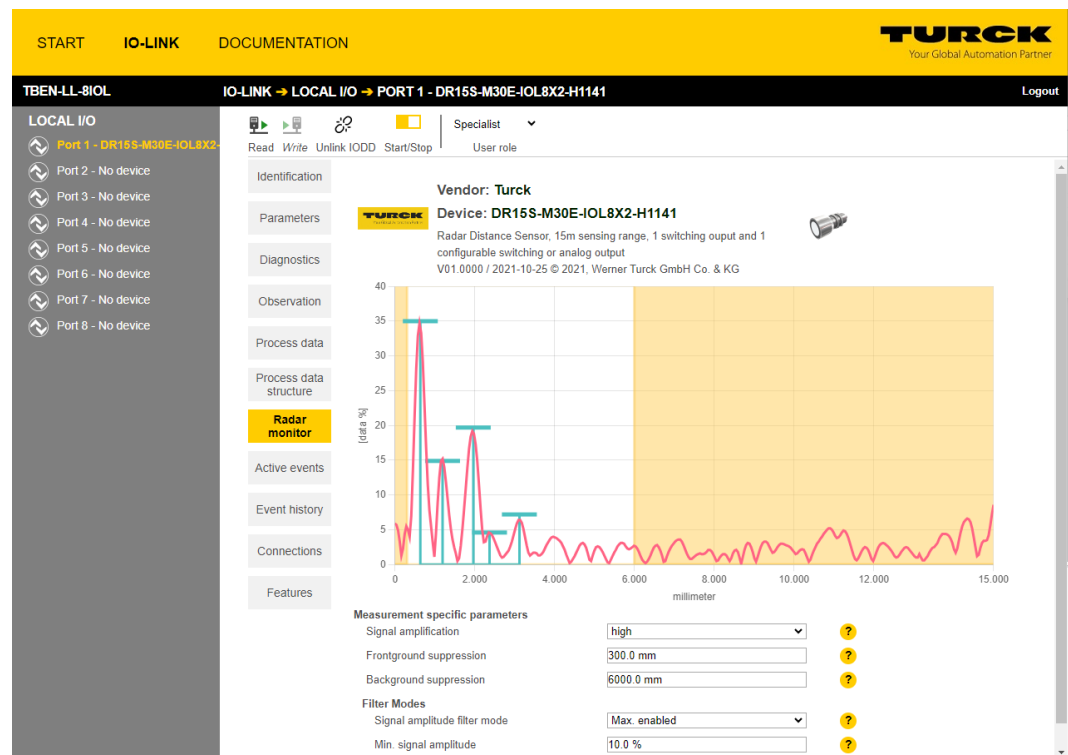
Fig. 114: Radar monitor
