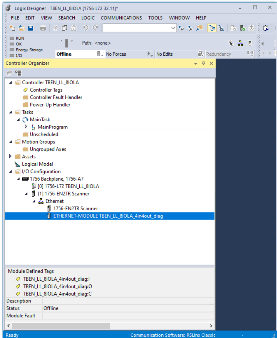
Fig. 70: Predefined configuration of TBEN-LL-8IOLA in the new project
