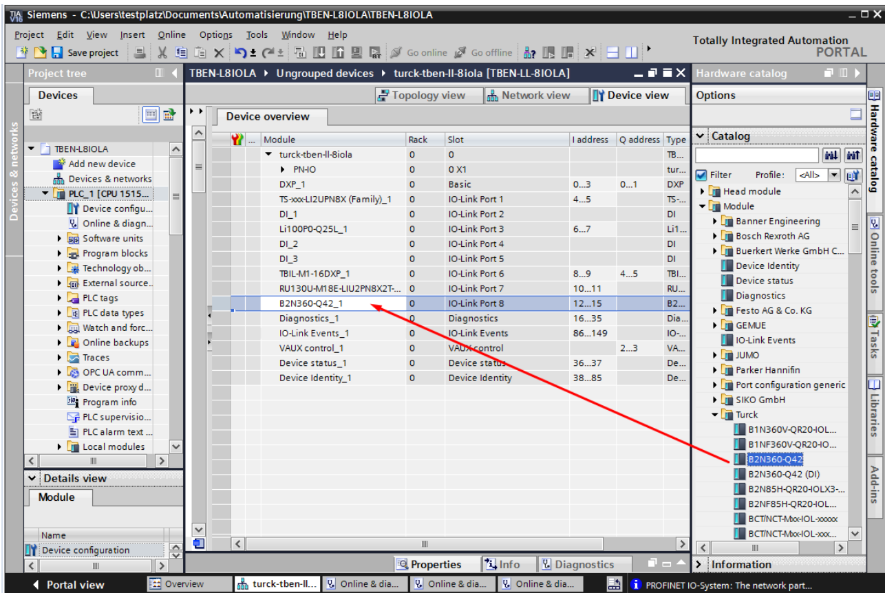
Fig. 43: TIA-Portal – configuring device slots
