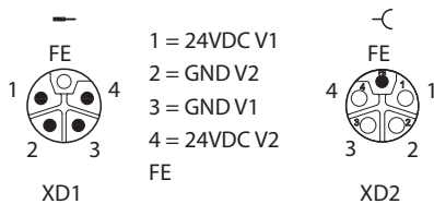
Fig. 23: Pin assignment power supply connectors
